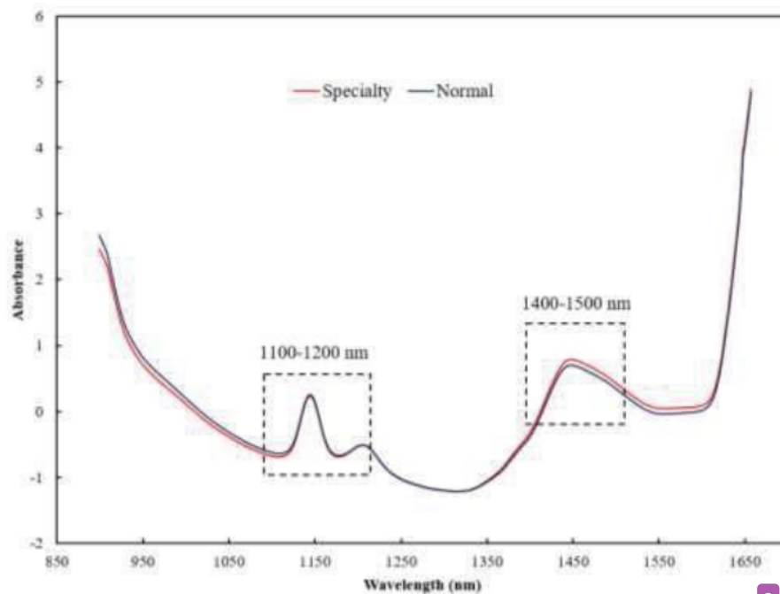
FIGURE 3. The average absorbance NIR preprocessed spectral data (MA 13s+SNV) of specialty and normal coffee samples in the range of 899-1657 nm.
