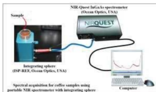
1 FIGURE 2. Spectral acquisition set up of coffee samples using portable spectrometer equipped with integrating sphere.
