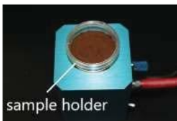
1 FIGURE 1. Sample holder for NIR diffuse reflectance spectral measurement.
