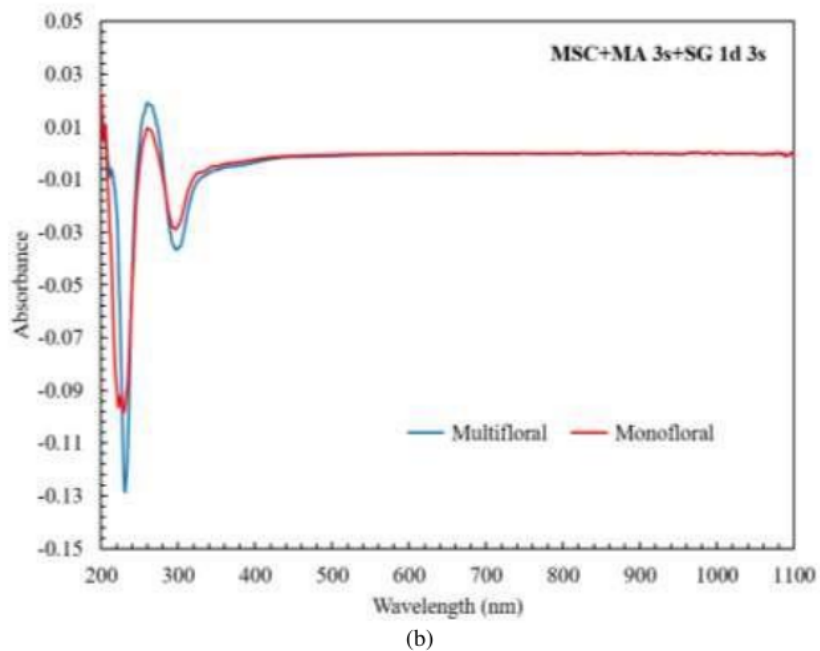
FIGURE 1. The average original (a) and transformed spectral data (b) of monofloral and multifloral honey samples in the wavelength of 190-1100 nm. 11
