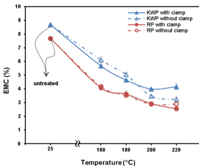
Fig. 3. Effect of temperature and clamping method on the change of EMC (KWP = Korean white pine; RP = royal paulownia)
