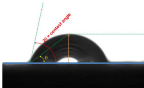
Fig. 2. Contact angle measurement using the half-angle method of drawing a line from the triphase point to the apex of the drop
