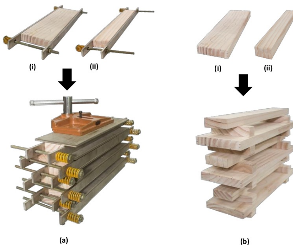
Fig. 1. Stacking of samples during heat treatment: (a) with a metal clamp, (b) without a metal clamp; samples for (i) physical properties, and (ii) mechanical properties evaluation
