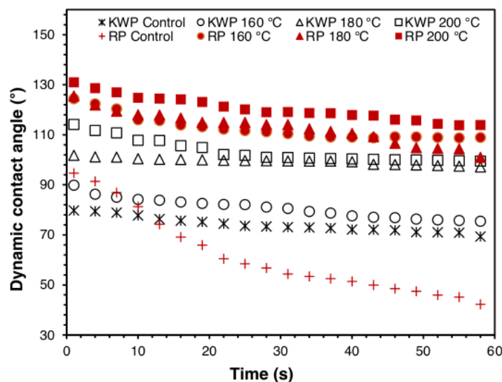
Fig. 4. Dynamic contact angle of Korean white pine (KWP) and royal paulownia (RP) before and after heat treatment
