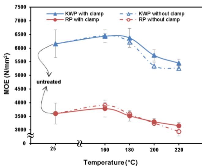
Fig. 8. Effect of temperature and clamping method on the change of MOE (KWP = Korean white pine; RP = royal paulownia)
