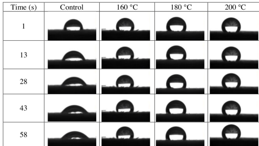
Fig. 6. Contact angles of royal paulownia before and after heat treatment
