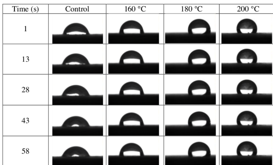
Fig. 5. Contact angles of Korean white pine before and after heat treatment
