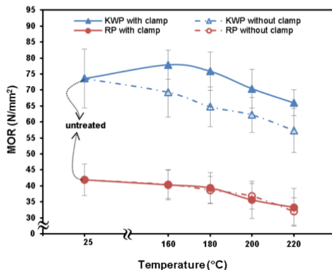
Fig. 7. Effect of temperature and clamping method on the change of MOR (KWP = Korean white pine; RP = royal paulownia)
