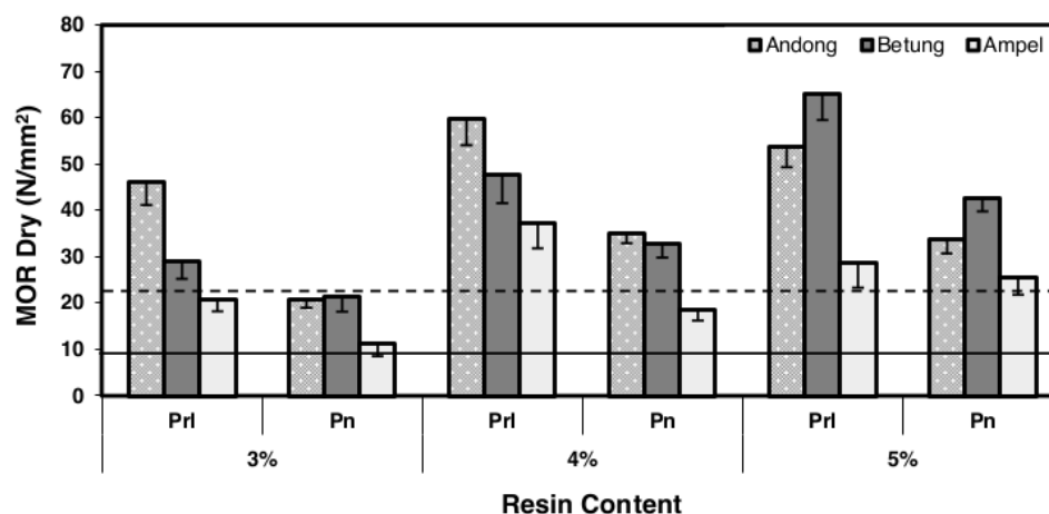
Fig. 6. Dry-state MOR parallel (pr) and perpendicular (pn) to the surface grain. Solid line: CSA O437.7 standard (grade O-1 OSB) for MOR perpendicular (= 9.42 N/mm 2 ); dashed line: CSA O437.0 standard (grade O-1 OSB) for MOR parallel (= 22.96 N/mm 2 )
