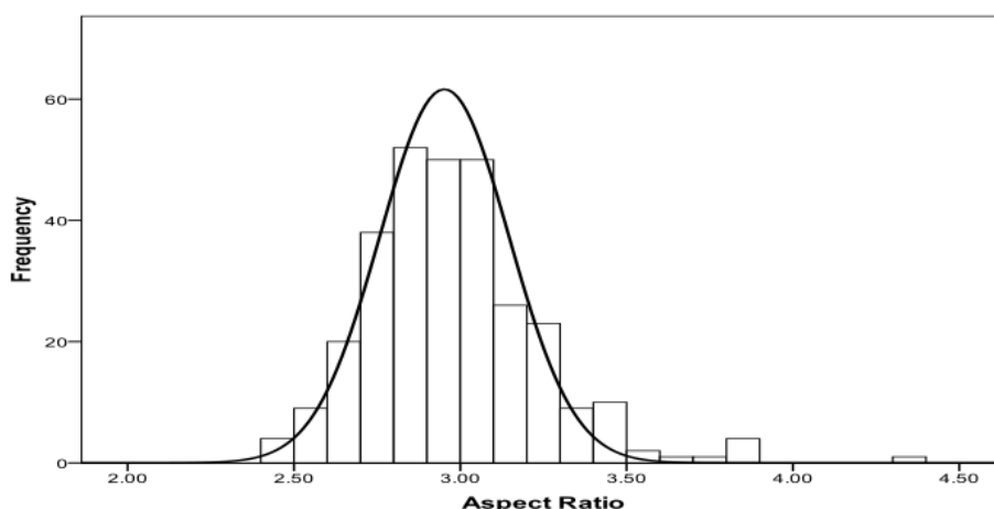
Fig. 2. Aspect ratio distribution of bamboo strands
