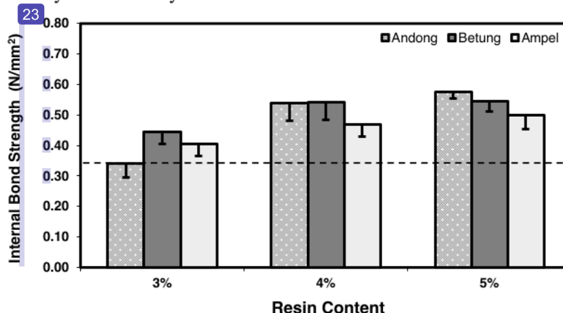
Fig. 10. IB values of OSBs from three bamboo species with various resin contents. Dashed line: CSA O437.0 standard (grade O-1 OSB) for IB (=0.34 N/mm²)
