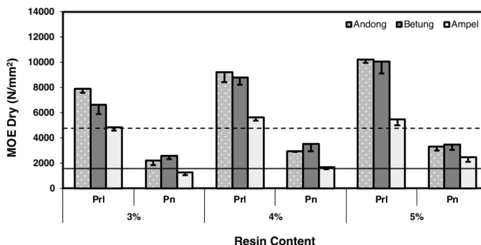
Fig. 8 Dry-state MOE parallel (pr) and perpendicular (pn) to the surface grain. Solid line: CSA O437.0 standard (grade O-1 OSB) for MOE perpendicular (= 1276 N/mm 2 ); dashed line: CSA O437.0 standard (grade O-1 OSB) for MOE parallel (= 4416 N/mm 2 )
