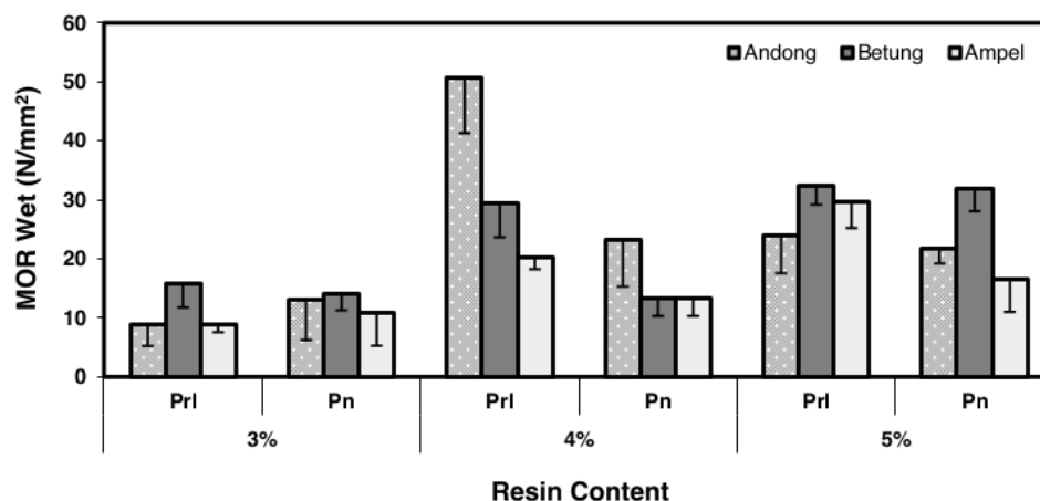
Fig. 7. Wet-state MOR parallel (pr) and perpendicular (pn) to the surface grain
