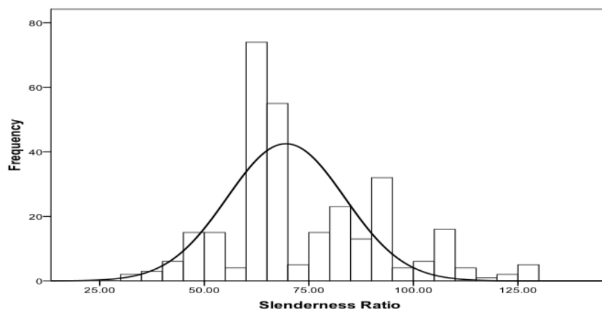
Fig. 1. Slenderness ratio distribution of bamboo strands
