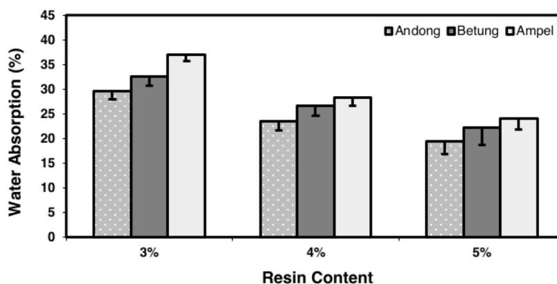
Fig. 4. Water absorption of OSBs from three bamboo species with various resin contents
