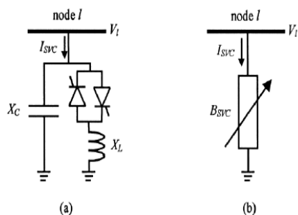
Gambar 1. Pemodelan SVC, (a) model firing angle SVC, (b) model total susceptance SVC[12]
