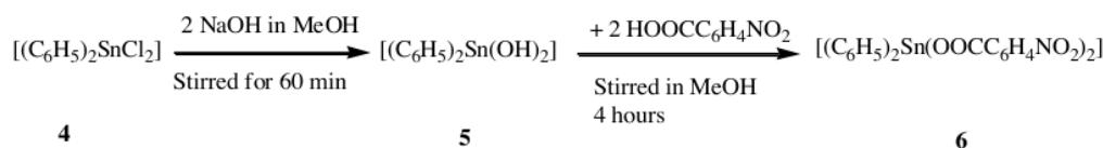
Fig. 1. Scheme for the preparation of organotin(IV) di-2-nitrobenzoate
