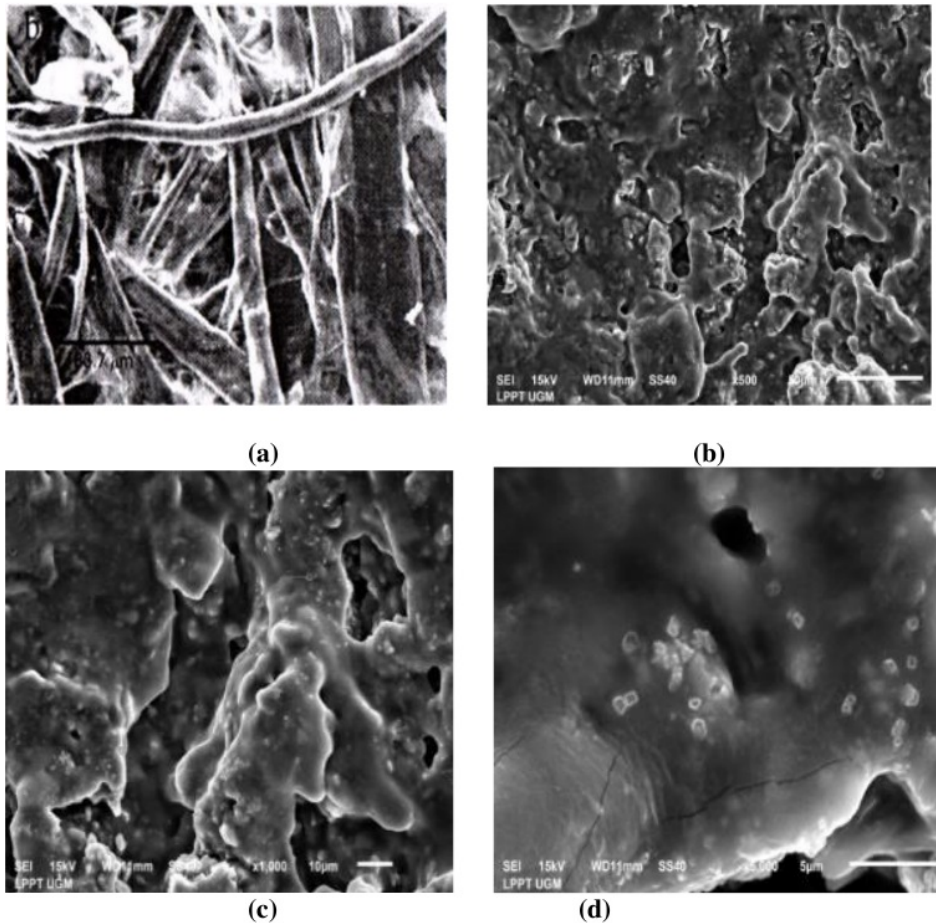
Figure 4. The results of SEM analysis (a) Cellulose, (b) CMC 500x magnification, (c) CMC 1000x magnification, and (d) CMC 5000x magnification
