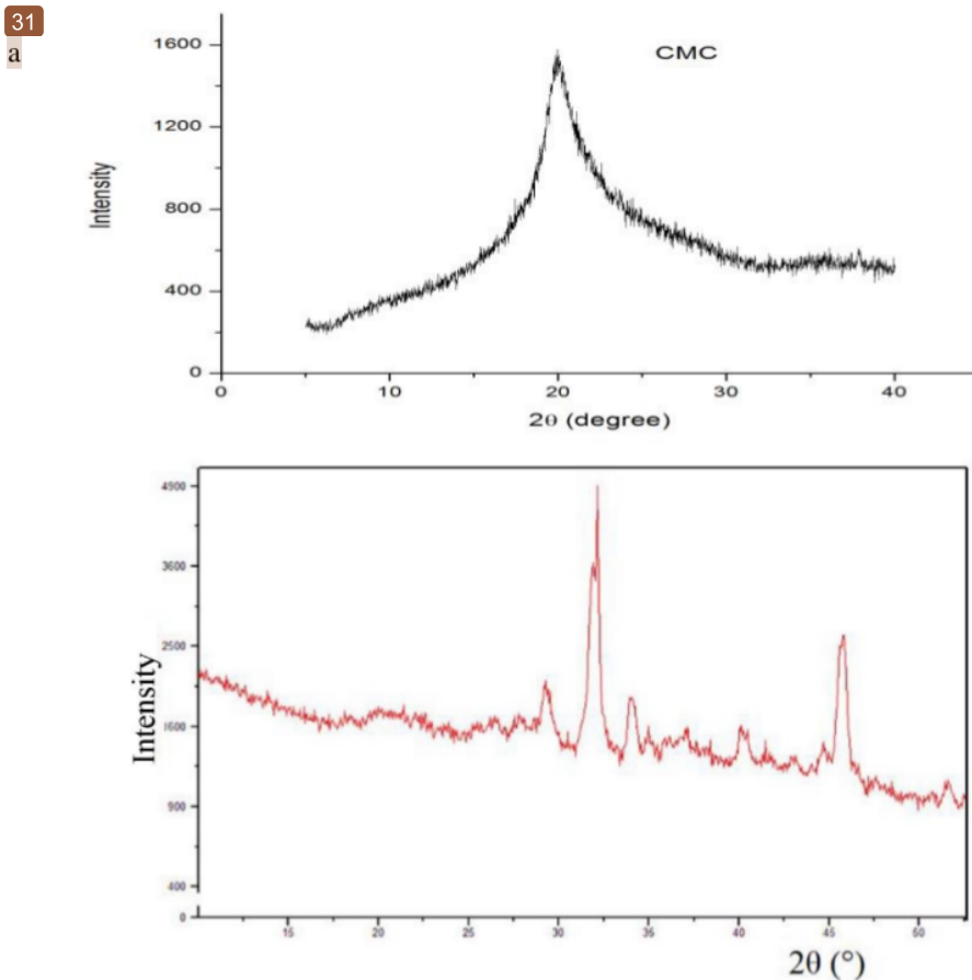
Figure 5. XRD diffraktrogram of (a) CMC standard, and (b) CMC research results.
