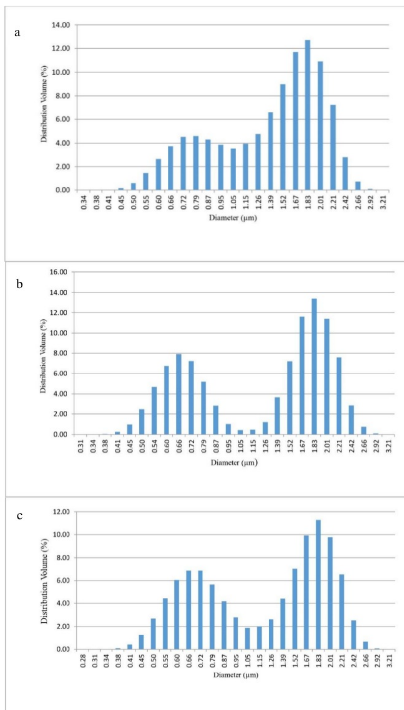
Figure 1. The result of PSA: (a) H 2 SO 4 concentration 45%, (b) H 2 SO 4 concentration 47%, (c) H 2 SO 4 concentration 49%.
