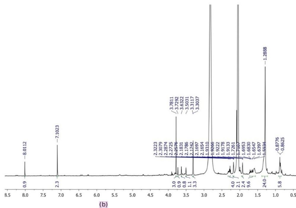
Figure 6. ^1\text{H} -NMR spectra of (a) \text{E}_2\text{zf} subfraction; (b) Reference compound (30).
