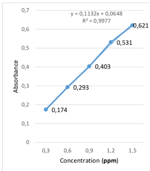
Figure 1. Chromium(VI) Standard Curve At Wavelengths of 540 nm.
