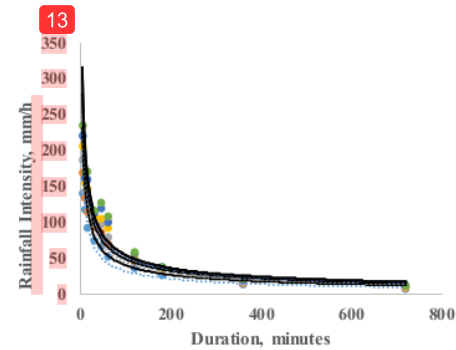
Fig. 3. IDF curve of the study area
