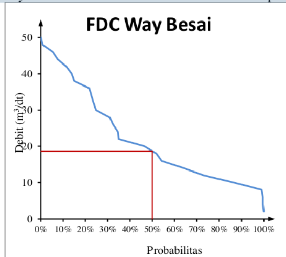
Gambar 10. Flow Duration Curve
