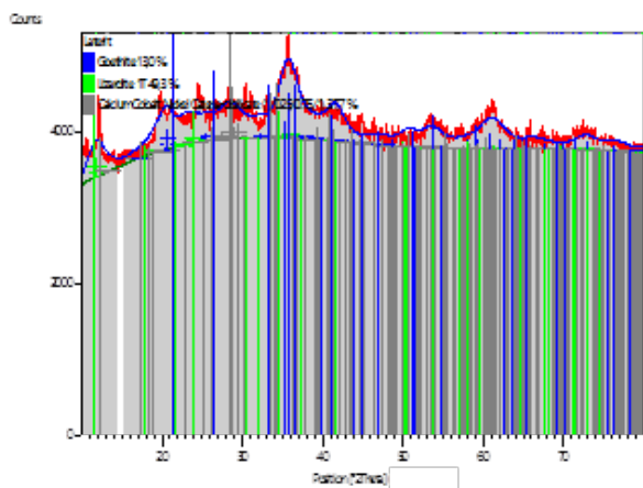
Figure 2. XRD analysis for Nickel Ore
