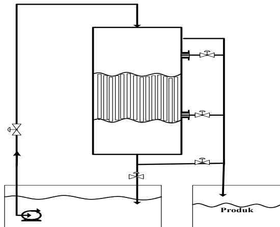
Figure 1. Batch recycling extraction scheme
