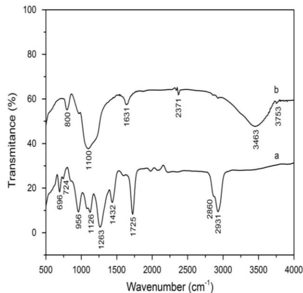
Figure 1. FTIR spectra of samples, (a) asphalt and (b) silica.
