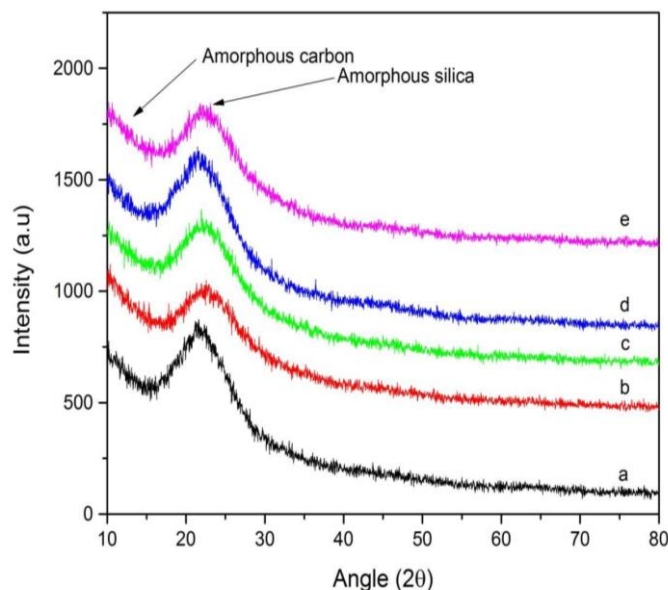
Figure 2. The X-ray diffraction patterns of the samples with the different calcination temperatures using CuK \alpha radiation, (a) 200 °C, (b) 250 °C., (c) 300 °C., (d) 400 °C and (e) 450 °C.
