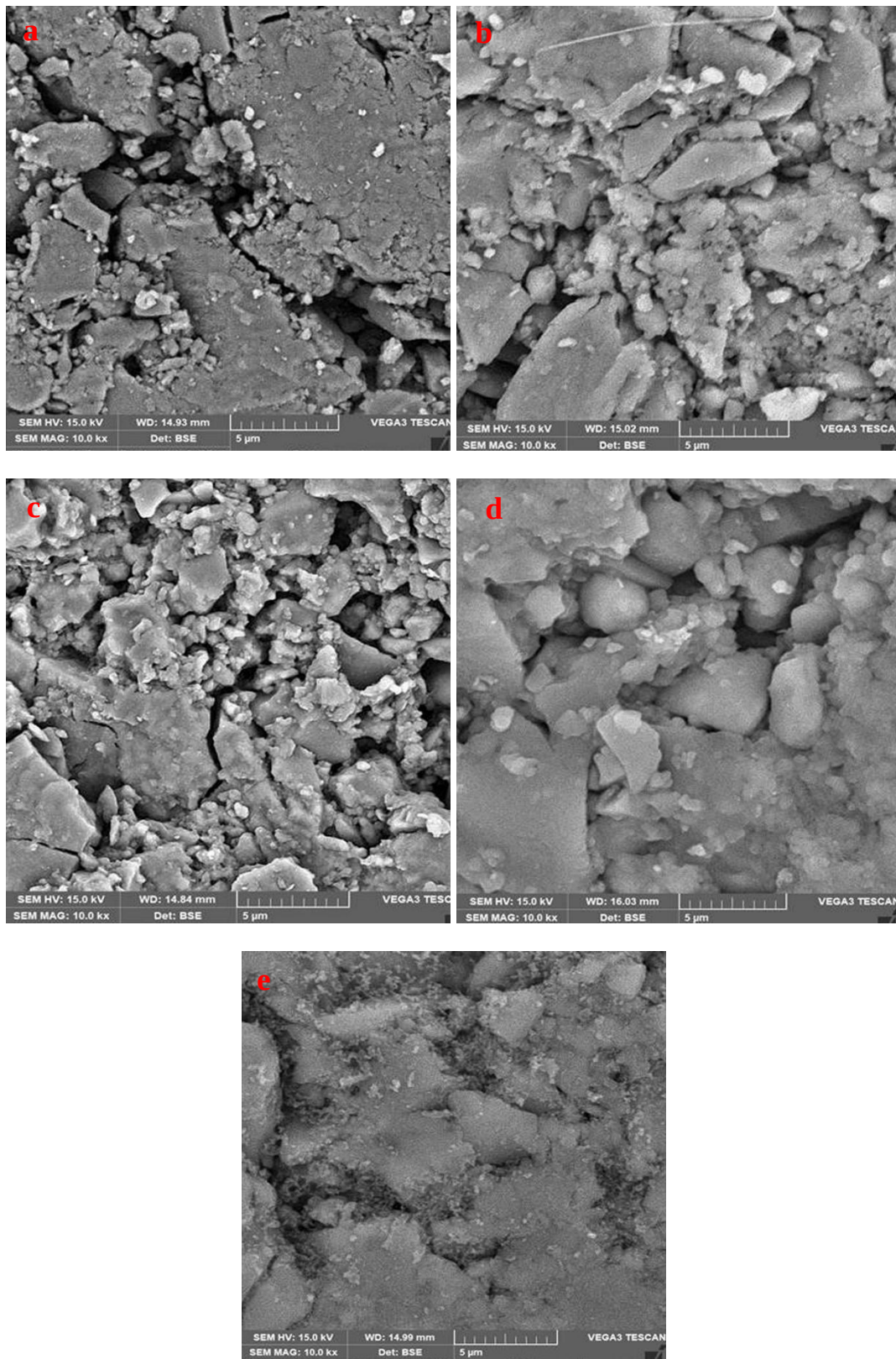
Figure 4. The scanning electron microscopy (SEM) images of the samples with different calcination temperatures (a) 200°C, (b) 250°C., (c) 300°C., (d) 400°C and (e) 450°C
