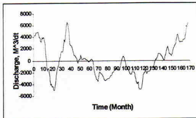
Figure 3. Marginal Loss Curve of Way Pengubuan
