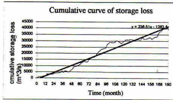
Figure 4. CumulativeStorage Loss Curve of Way Besai
