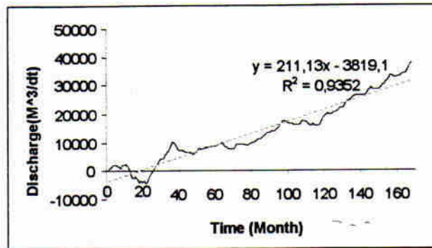
Figure 2. Cumulative storage loss of Way Pengubuan
