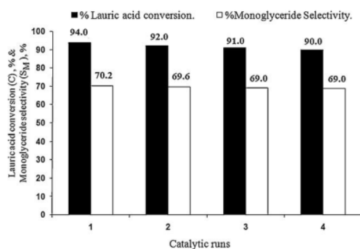
Fig. 9. Lauric acid conversion and monoglyceride selectivity shown by HSO 3 SBA-15 catalyst when used in four successive runs.
