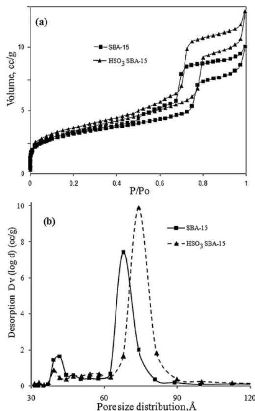
Fig. 4. N 2 adsorption-desorption isotherm curves: (a) and pore size distribution curves: (b) of SBA-15 and HSO 3 SBA-15 catalyst.
