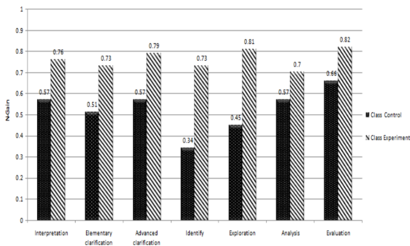
Figure 3 Graph of n-gain value calculation of critical thinking indicator
