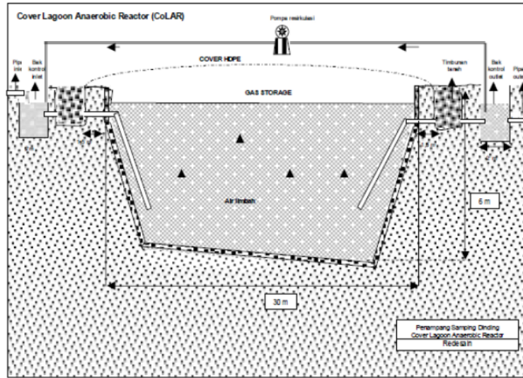
Gambar 2. Desain CoLAR (Isdiyanto & Hasanudin, 2010).
