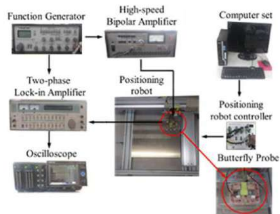
Figure 8. Experimental set-up.
