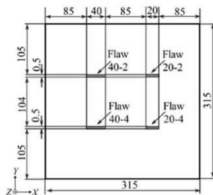
Figure 7. Specifications of test piece (units in mm).
