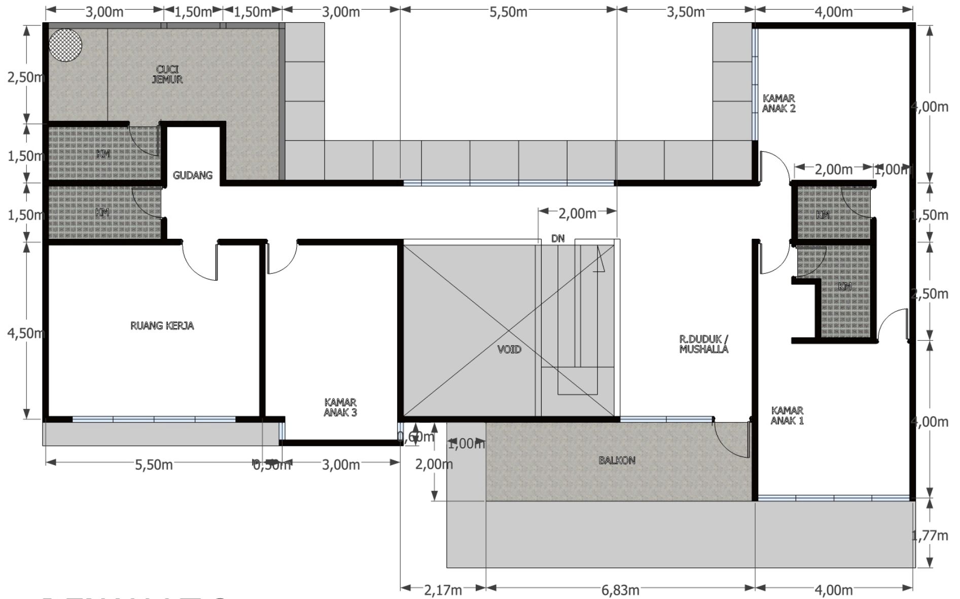
DENAH LT.2
