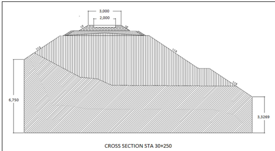
Figure 2. Cross section in the location of study
