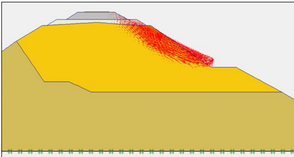
Figure 5. Total soil displacement due to landslides
