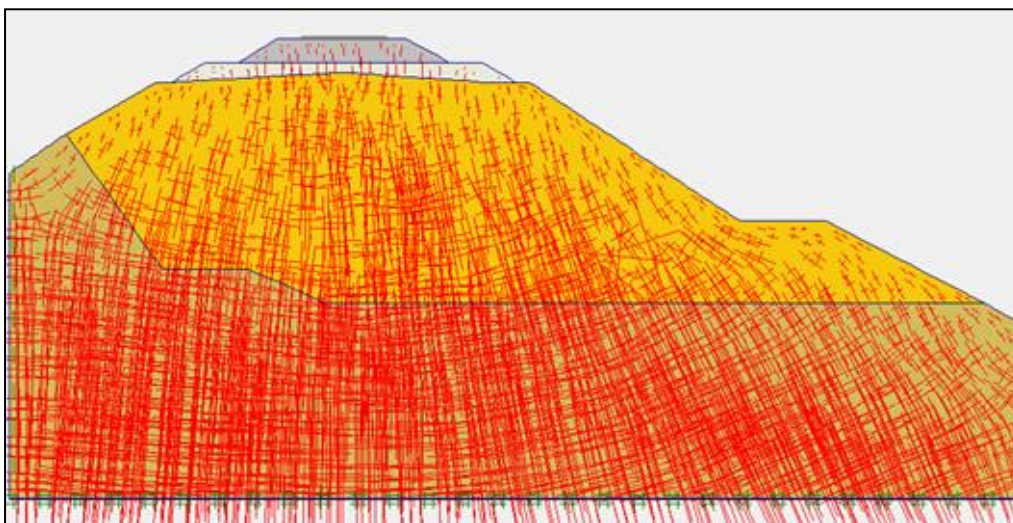
Figure 6. Effective stress illustration
