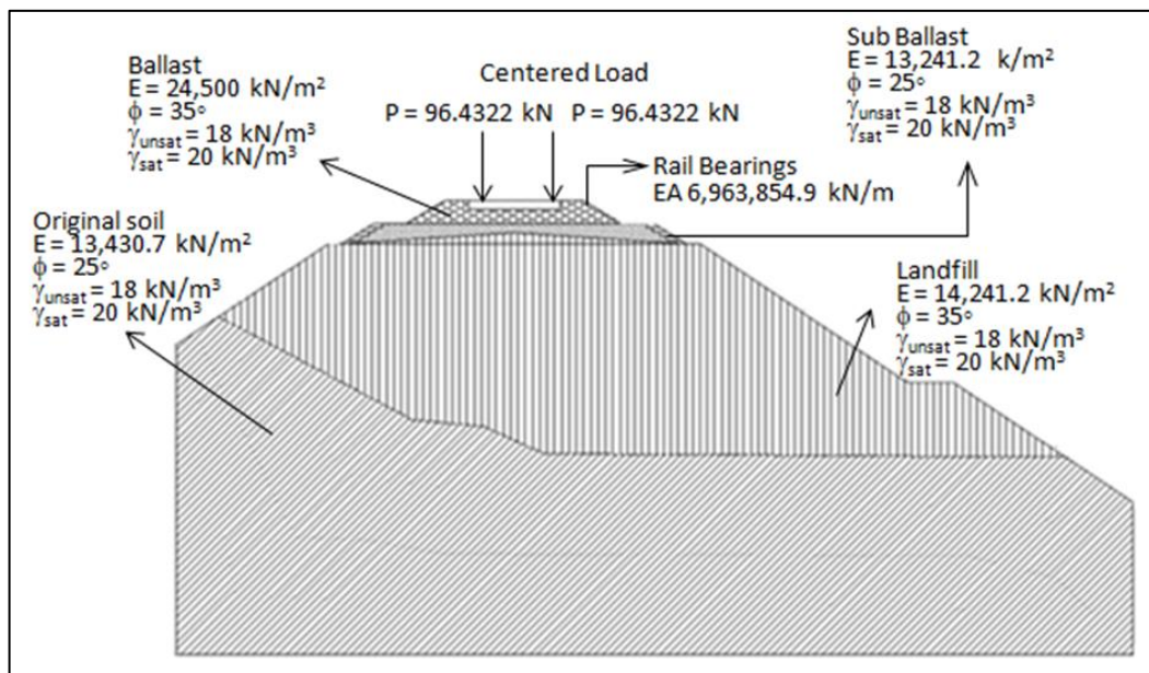
Figure 3. Force distribution in the cross section studied
