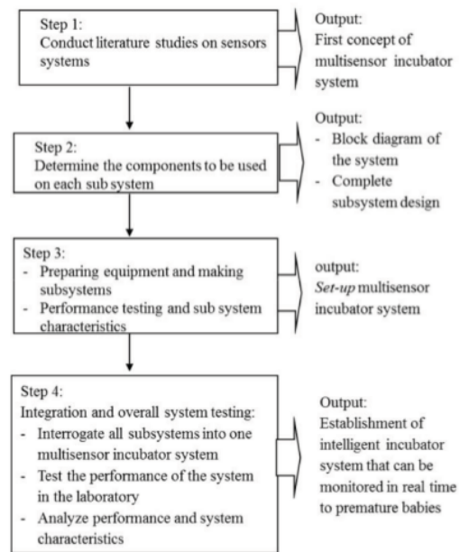
Fig. 3. Research Steps
