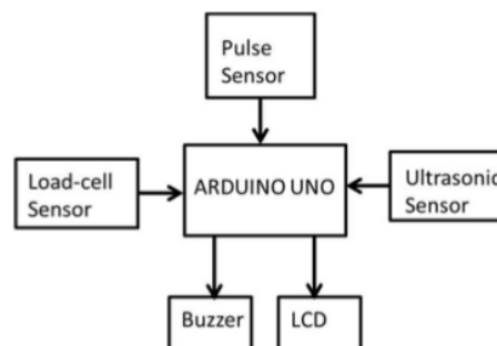
Fig. 1. Block diagram of multisensor system
