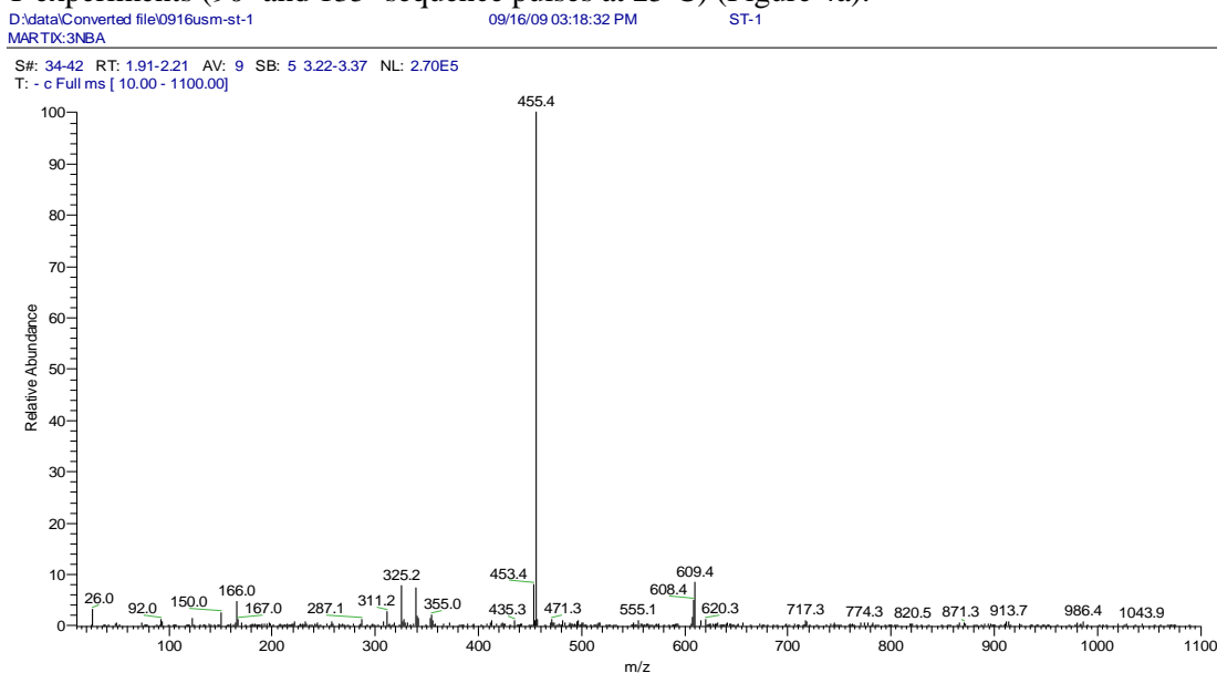
Figure 1. FABMS spectrum of 1 (negative-ion mode)
