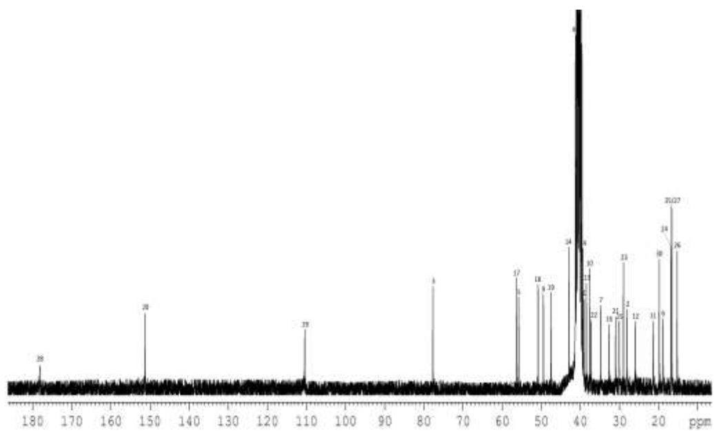
Figure 3. ^{13}\text{C} NMR spectrum of 1 (75 MHz, \text{DMSO-}d_6 )
