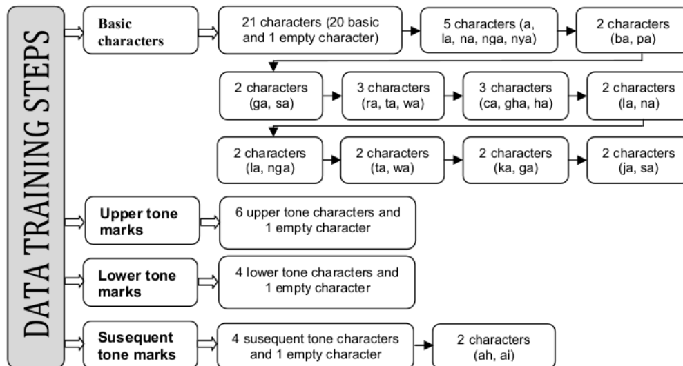
Figure 7. Data training steps.
