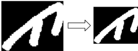
Figure 5. Resizing process.
