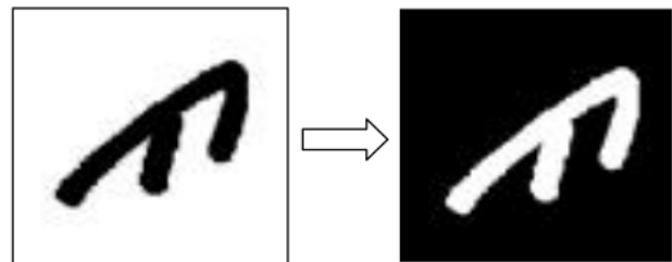
Figure 3. Inverting process.
