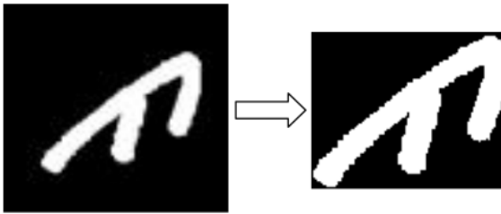
Figure 4. Cropping process.
