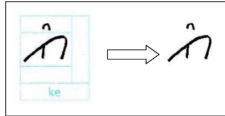
Figure 1. Binarization process.
