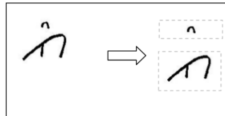
Figure 2. Slicing process.
