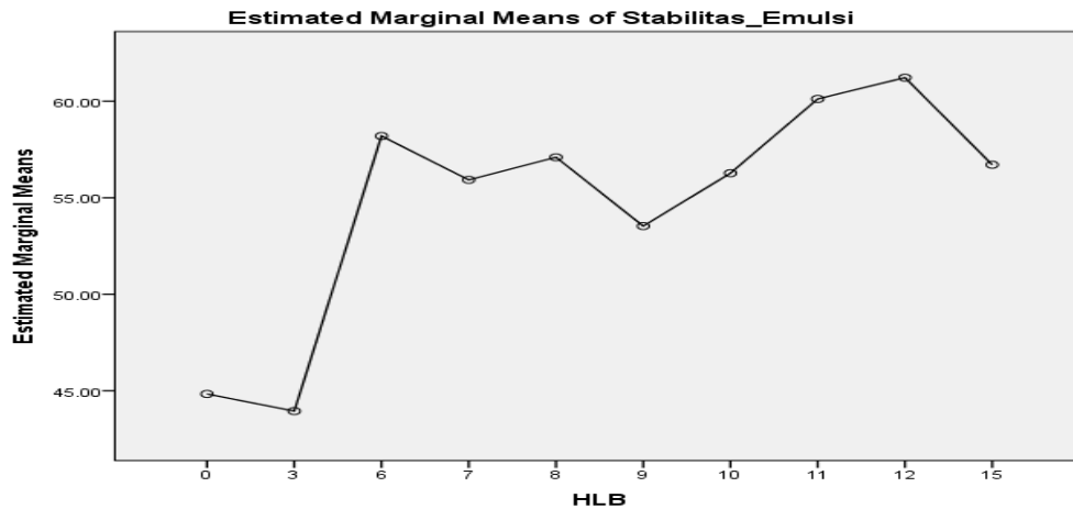
Figure 1. Emulsion stability values of coconut milk (without dilution of water) with addition of the emulsifier mixture with HLB values of 3 up to 15 (HLB 0 is coconut milk control without the addition of an emulsifier)
