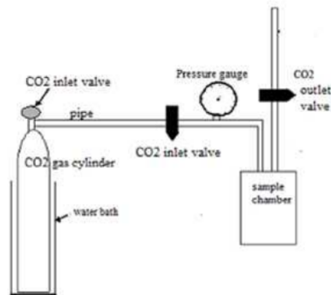
Figure 1 The set-up of the experimental apparatus (Saputra, 2006).
