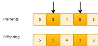
Figure 3: Illustration of swap mutation operation
