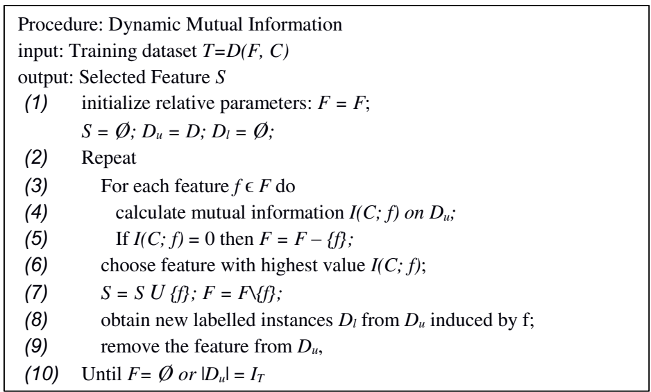
Figure 1. Procedure dynamic mutuali information
