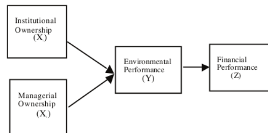
Figure 2. Framework
