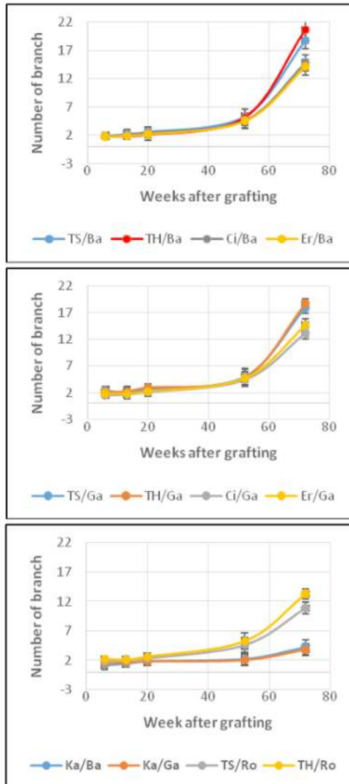
Figure 2. Number of primary branch Remarks: TS: Tugusari, TH: Tugu Hijau, Ci: Ciari, Er: Ersad, Ba: Bakir, Ga: Garudak (Robusta), Ro: Robinson (Liberica), Ka: Kartika (Arabica) rootstock genotypes. Genotypes of Ciari and Ersad performed slower growth when grafted onto Bakir and Garudak. Genotypes of Tugu Sari and Tugu Hijau showed slower growth when grafted onto Robinson (Liberica). Without total pruning of Robusta rootstock, Kartika/Robusta grafting branches showed significantly slow growth and maturity.
