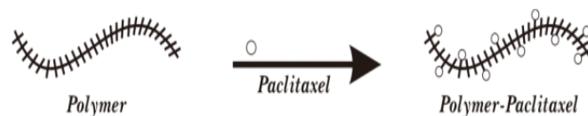
Figure 3. Paclitaxel encapsulation scheme [17]
