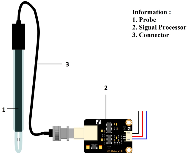
Fig. 1. EC sensors are integrated into the microcontroller
