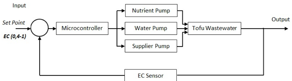
Fig. 1. EC sensors are integrated into the microcontroller
