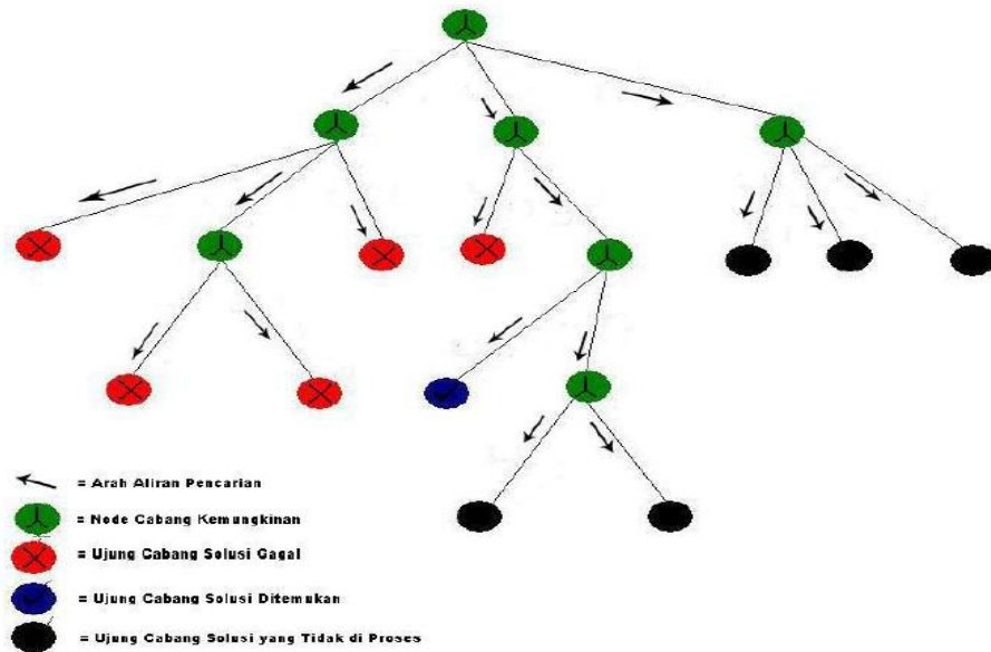
Gambar 3.5. Runtime penelusuran tracking guess kage-bunshin
