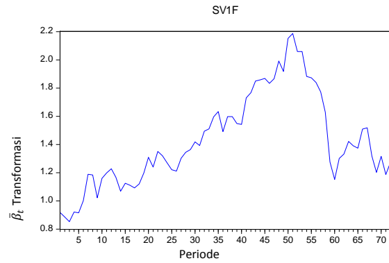
Gambar 6. Plot \beta_t Data Transformasi
