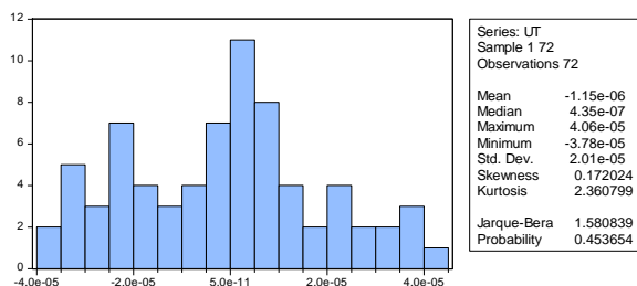
Gambar 7. Histogram Residual Data Transformasi
