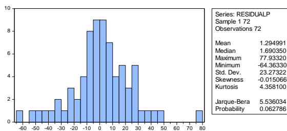
Gambar 4. Histogram Residual Data
