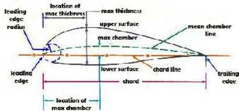
Figure 6. Parameters of NACA airfoil
