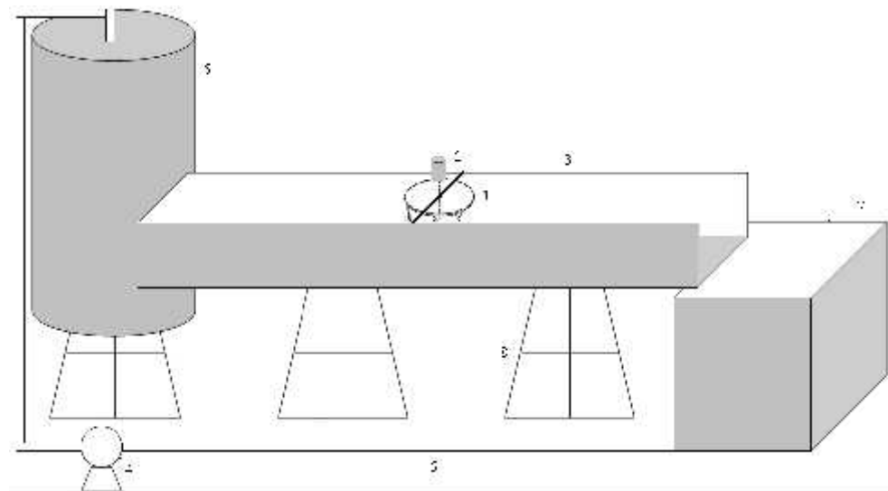
Figure 4. Schematic of testing equipment system
