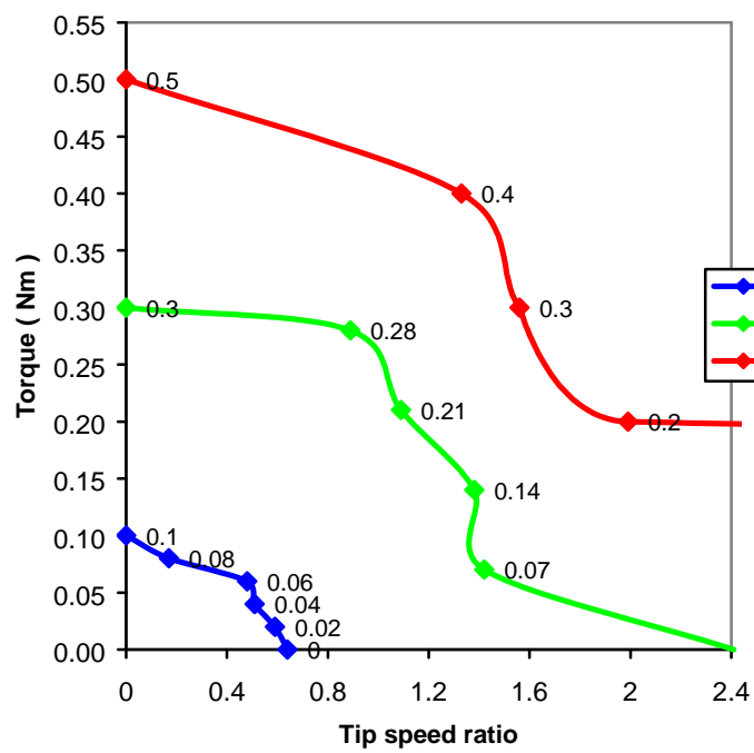
a. Influence of volume flow rate on the torque
