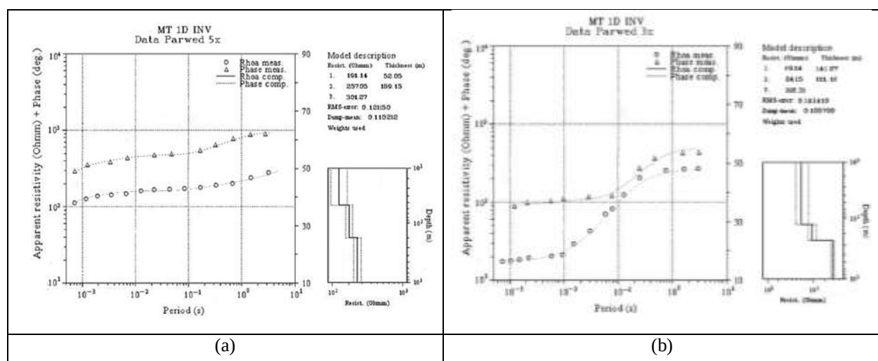
Figure 3. The 1-D inversion window uses MTINV from 5x data with the smallest error acquisition with 3 layers (a), 1-D inversion results use MTINV from 3x data which shows the first layer is thicker than in 5x data (b).
