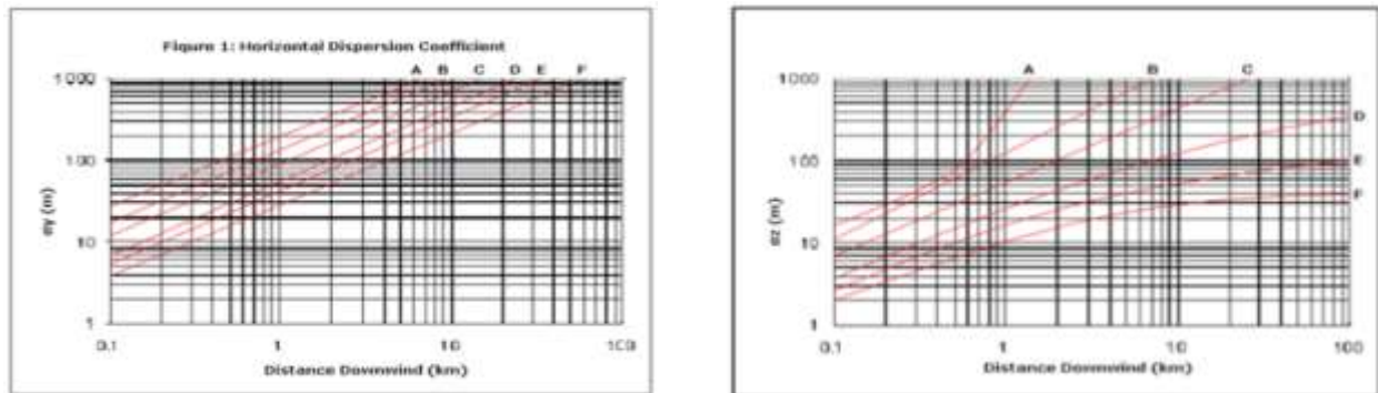
Gambar 3. Horizontal Dispersion dan Vertikal Dispersion Coefficient ( \sigma_z )
