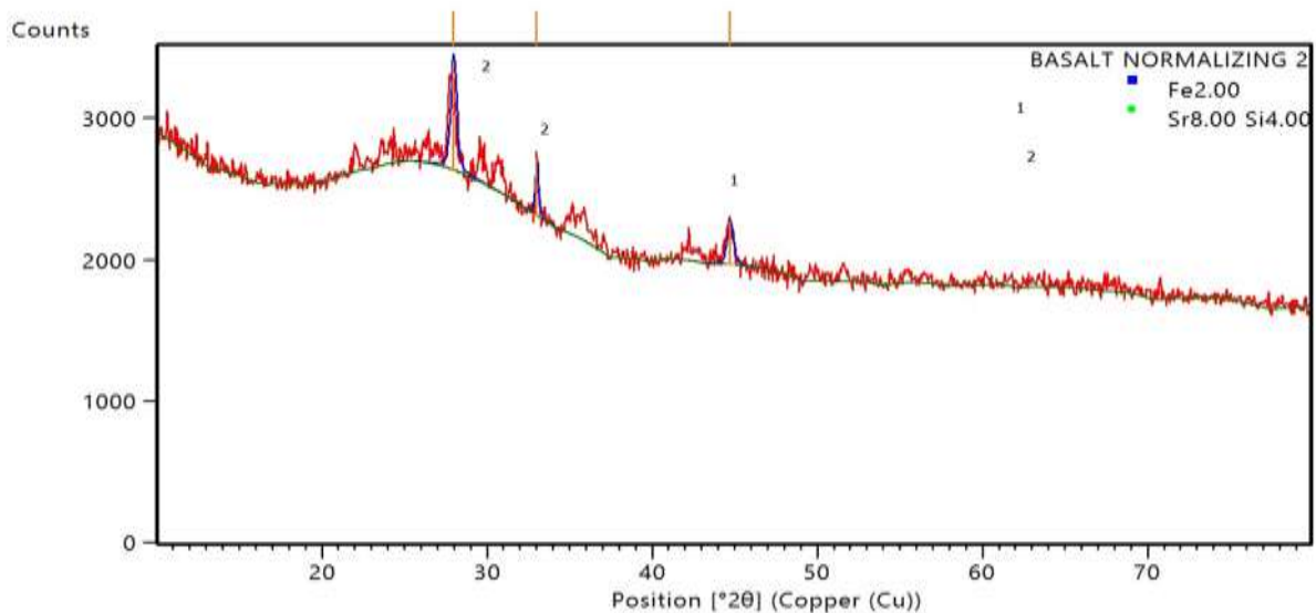
Gambar 4. Hasil analisa XRD pengecoran basalt pendinginan normalizing
