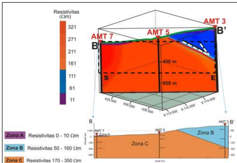
Figure 4. The division of zones into 3, the highly conductive zone is zone A with resistivity 0 to 10 ohmmeter that is located on the southwest side of the study area, while the conductive zone is written zone B with resistivity 50 - 160 ohmmeter on the northeast side of the study area.
