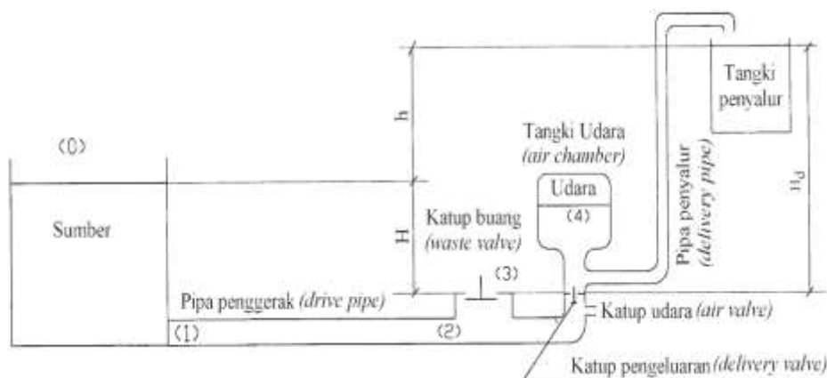
Gambar 2. Instalasi pompa hydraulic ram pump
