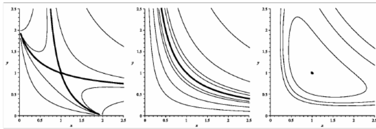
Figure 2. The bifurcation (or change of stability) of the critical point of F_1 as \mu passes 0.
