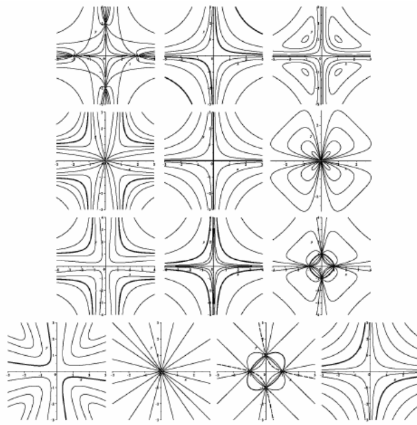
3 Figure 1. In this figure, we have plotted some level sets of the function F_k , k = 1, \dots, 7 , for various values of \mu . The diagrams in the first row are the level sets of F_1 for \mu = \frac{1}{4} , 0 , and -\frac{1}{4} , from left to right, respectively. The diagrams in the second row are the level sets of F_2 for \mu = 1, 0 , and -1 , from left to right, respectively. Lastly, the diagrams in the third row are of F_3 for \mu = 2, 0 and -\frac{1}{4} . The diagrams in the fourth row are the level sets of F_4, F_5, F_6 , and F_7 , respectively.
