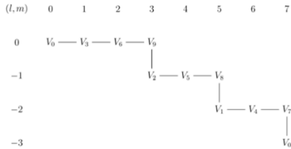
Figure 7. For the case where z_1 = 3 and z_2 = 7 .
