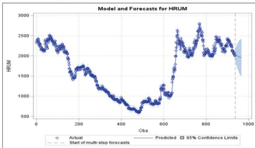
Figure 7: Prediction and forecasting of HRUM energy data
