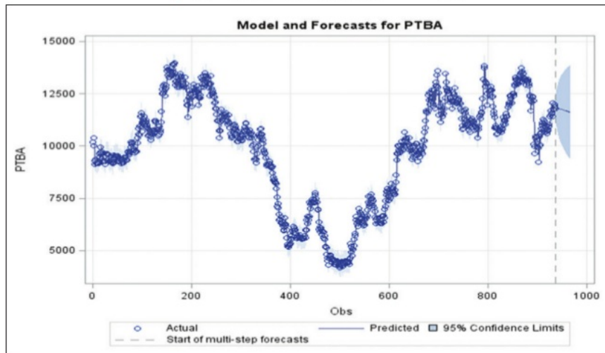
Figure 6: Prediction and forecasting of PTBA data
