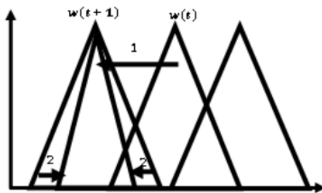
Fig. 3. Update Codebook Vector When Classification is False
