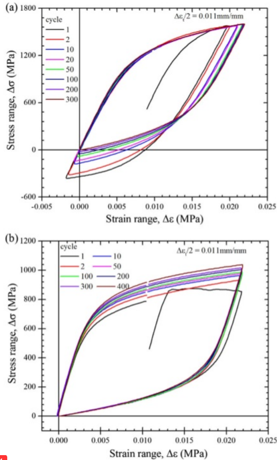
1 Fig. 6. Plots of the hysteresis loops with matching upper branches during symmetrical strain cycling with a strain amplitude of 0.011 mm/mm: (a) the as-received AISI 4140 steel and (b) the AS.
