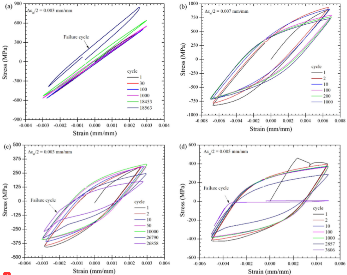
1 Fig. 5. Plots of the hysteresis loops obtained from the LCF tests at different strain amplitudes: (a and b) the as-received AISI 4140 and (c and d) the AS.
