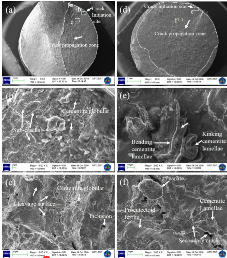
1 Fig. 14. SEM of fracture surfaces from the samples tested under LCF at a strain amplitude of 0.009 mm/mm; (a–c) the as-received AISI 4140 and (d–f) the AS.
