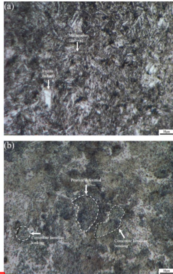
1 Fig. 7. Optical micrograph of (a) an RS sample and (b) an AS sample after LCF testing at a strain amplitude of 0.009 mm/mm.
