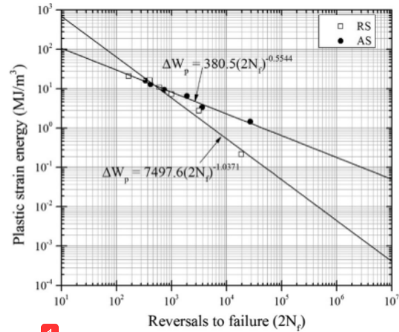
1 Fig. 13. LCF plots based on plastic strain energy with reversals to failure ( 2N_f ) for strain amplitudes ranging from 0.003 to 0.013 mm/mm.
