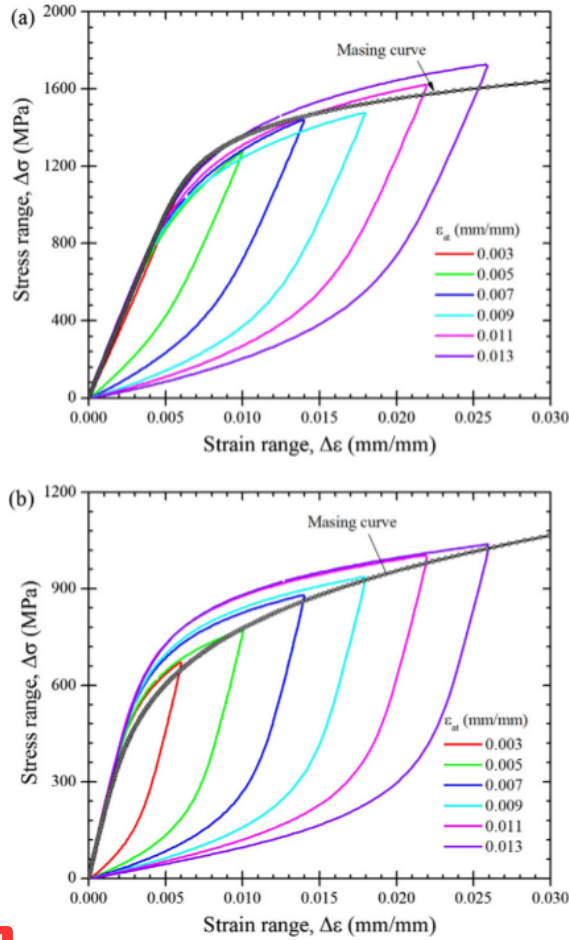
1 Fig. 9. The non-Masing and near-Masing curves superimposed on hysteresis loops at half cycles with a common compressive tip for (a) the as-received AISI 4140 and (b) AS.
