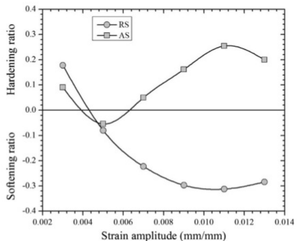
1 Fig. 8. The cyclic softening/hardening ratios of the RS and AS from the LCF tests at a constant strain rate of 0.005 s -1 .
