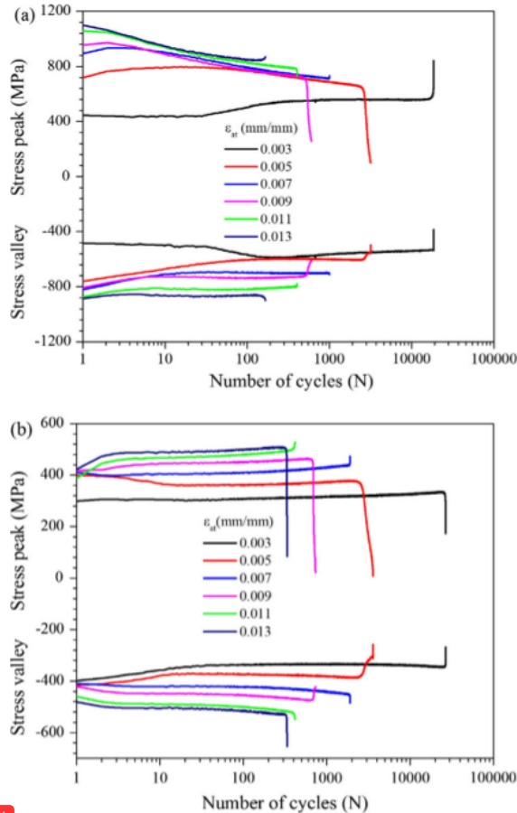
1 Fig. 4. Cyclic stress response during LCF tests: (a) the as-received AISI 4140 steel and (b) AS.
