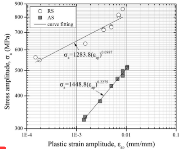
1 Fig. 10. Influence of annealing treatment on the cyclic stress amplitude and the plastic strain amplitude obtained from the LCF tests at different strain amplitudes.
