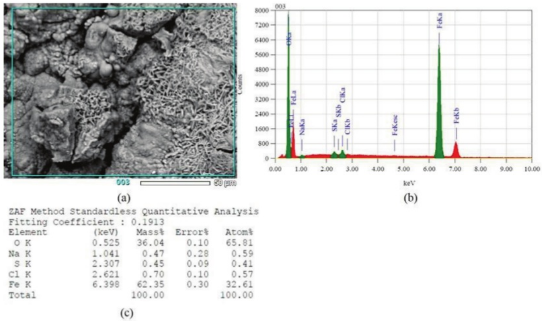
FIGURE 6. (a) SEM surface morphology of AISI 1020 steel with mixtures of 70/30 wt.% (NaCl/Na 2 SO 4 ) deposit after hot corrosion of 49 h at 700°C (b) its EDS spectrum, and (c) EDS quantitative analyses results in part (a)
