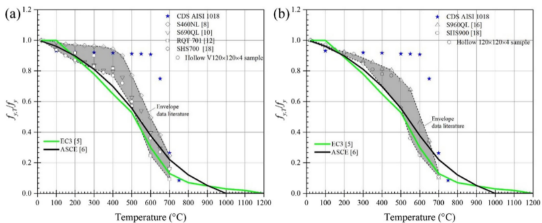
1 Fig. 14. Comparison of the reduction factor-temperature relationship of the yield strength under transient-state conditions for different steel grades (a) f_y < 700 and (b) f_y > 700 .
