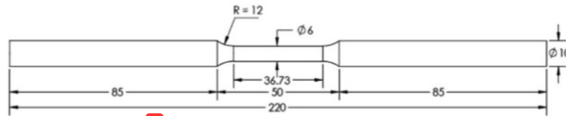
1 Fig. 1. Dimensions of the tensile specimens (all in mm).
