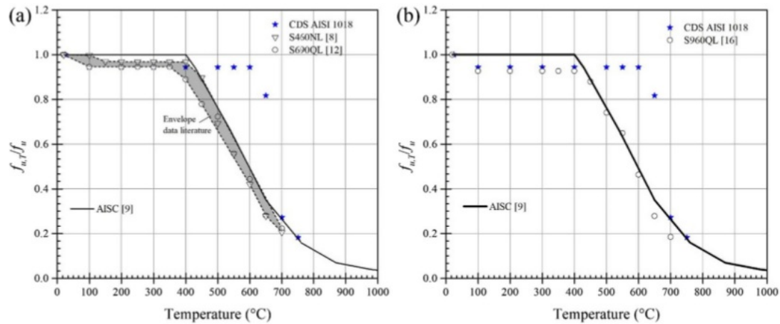
Fig. 15. Comparison of the reduction factor–temperature relationship of the ultimate strength under transient-state conditions for different steel grades (a) f_u < 700 and (b) f_u > 700 .
