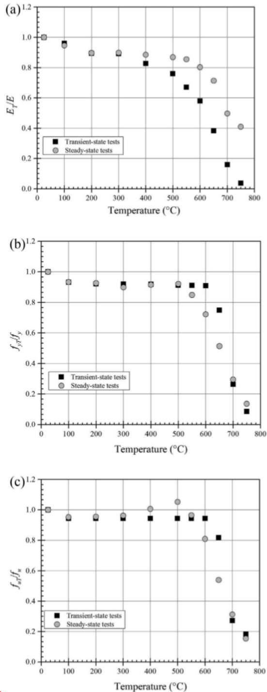
1 Fig. 9. Comparisons of the reduction factor-temperature relationship: (a) elastic modulus, (b) yield strength, and (c) ultimate strength under steady- and transient-state conditions.
