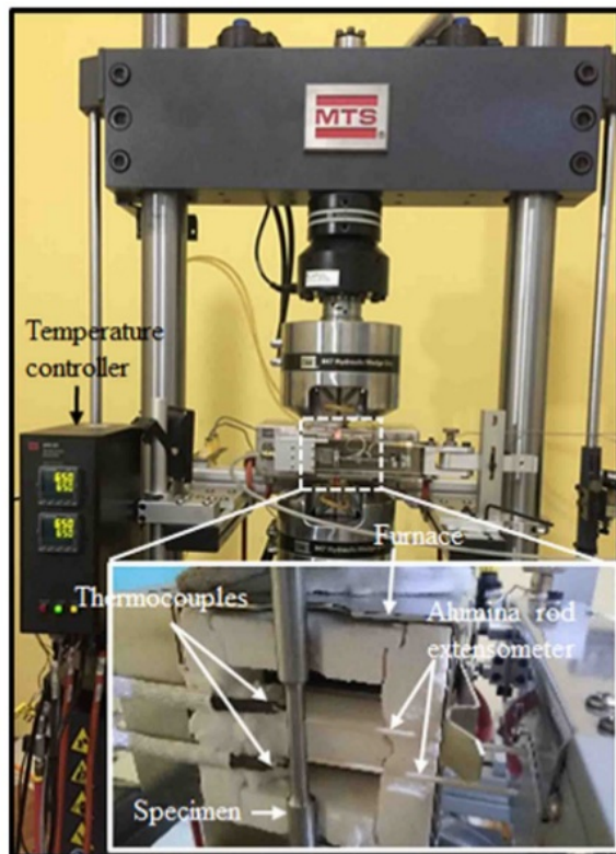
1 Fig. 3. Detailed view of the experimental setup: positions of the thermocouples and mounting extensometer on the specimen.
