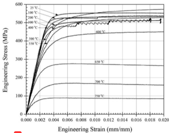
Fig. 5. Stress-strain curves of CDS 1018 at elevated temperatures.
