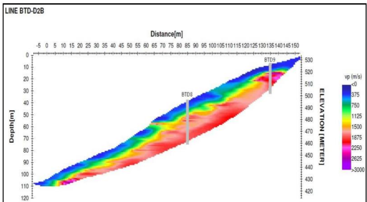
Gambar 6. Penampang seismik line BT-D2B
