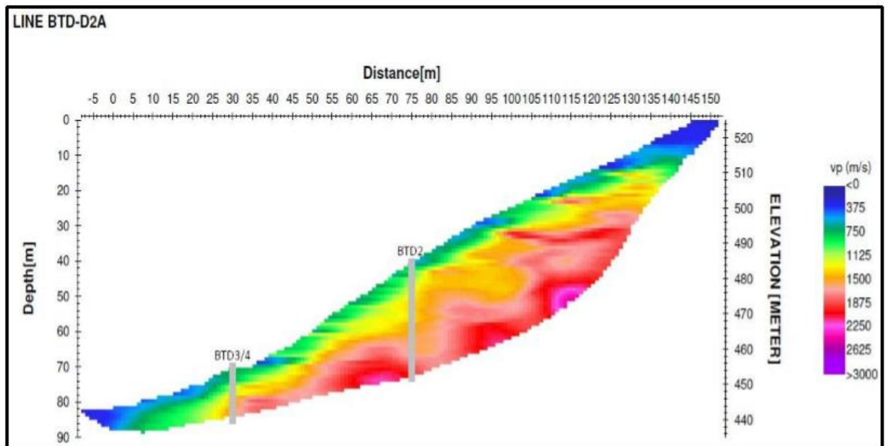
Gambar 5. Penampang seismik line BT-D2A
