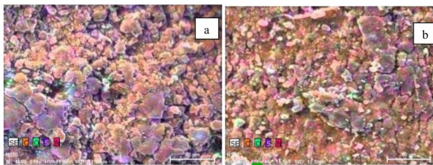
5 Figure 4. Mapping of Element from EDX Result: (a) NR/CB (N220) (b) NR/CB (N550)
