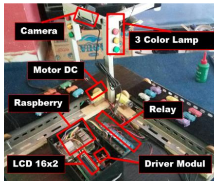
Figure 5. Hardware model
