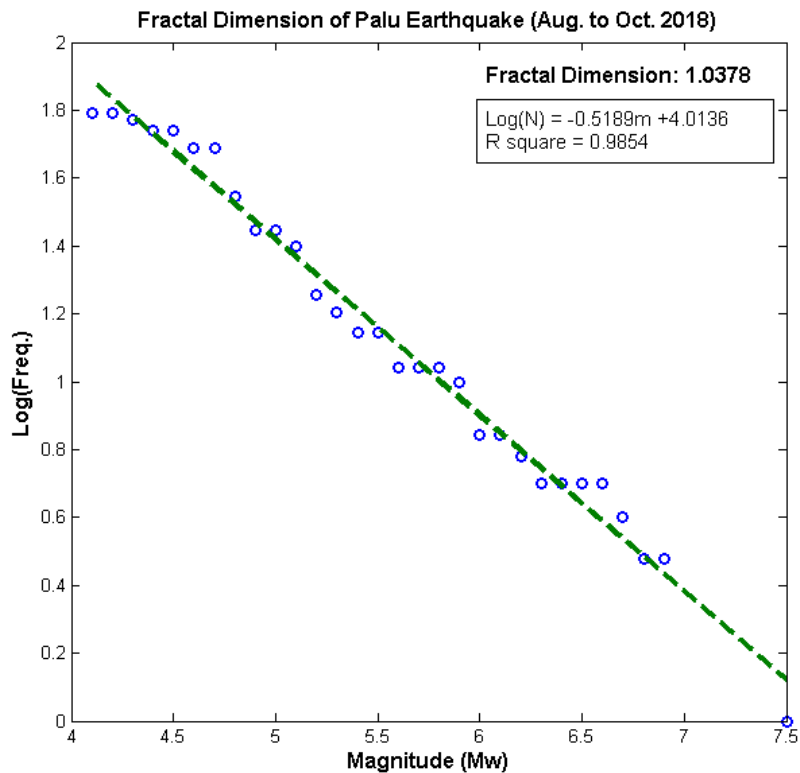
Figure 7. Fractal dimension of Palu earthquake from August to October 2018
