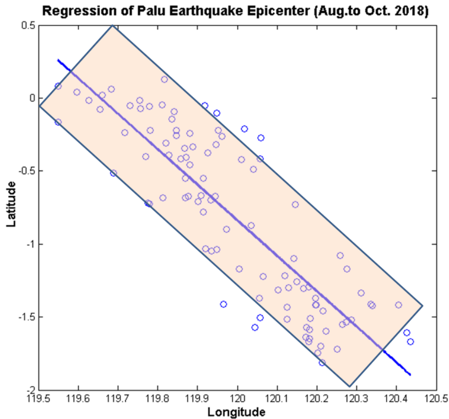
Figure 8. Estimated of line fracture of the Palu earthquake in August to October 2018. There are two segments of the earthquake distribution of each upper and lower segment in the PKF zone. The results of the epicenter linearization of the PKF zone in that period are shown in Figure (8), indicate the pattern of seismicity in the Southeast - Northwest direction that was estimated as rupture line segments along the PKF zone.
