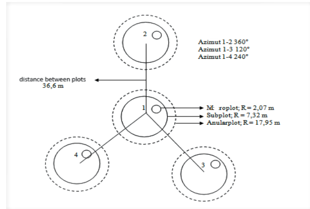
Figure 1 Cluster plot design
