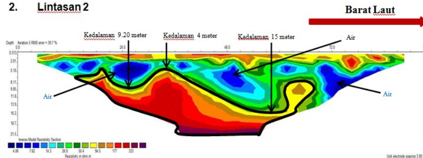
Gambar 31. Lintasan 2 dipole-dipole PT. Kereta Api Indonesia
