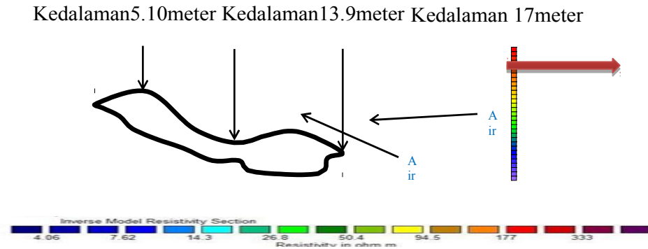
Gambar 30. Lintasan 1 dipole-dipole PT. Kereta Api Indonesia
