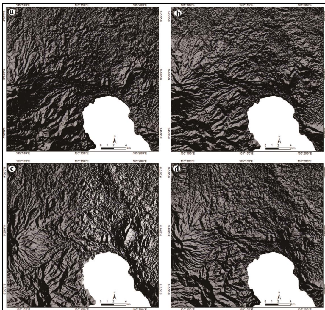
Figure 3. Four azimuth directions from the hill-shade analyze, a) N 315°E, b) N 0°E, c) N 45°E, and d) N 90°E. Four azimuth direction have done combine for produce hill-shade exactly is representative real geological condition surface.
