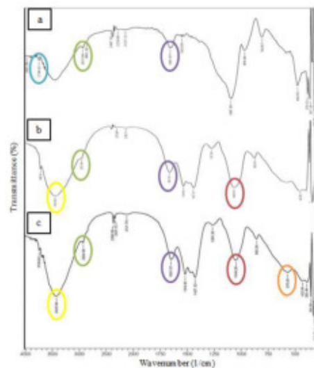
Fig 1. Infrared spectra of the (a) Porphyridium sp. (b) HA-S, and (c) HA-SM.
