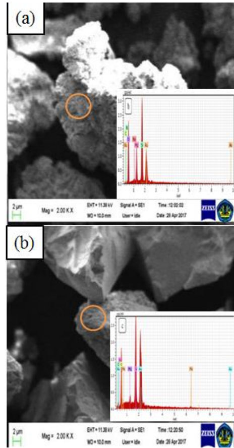
Fig. 2. SEM images and EDX spectra of (a) HA-S and (b) HA-SM.
