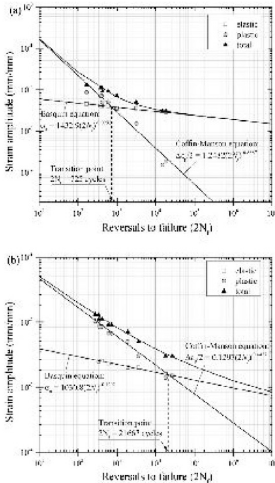
Fig. 11. Fatigue strain-life curves and calibration curves using the Coffin-Manson-Basquin relationship for (a) the as-received AISI 4140 steel and (b) the AS.
