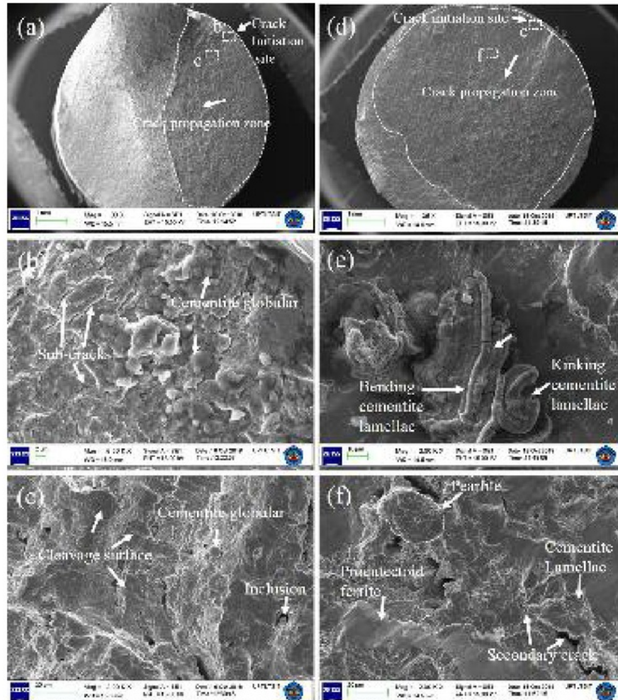
Fig. 14. SEM of fracture surfaces from the samples tested under LCF at a strain amplitude of 0.009 mm/mm; (a–c) the as-received AISI 4140 and (d–f) the AS.
