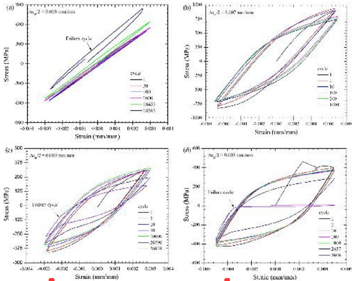
Fig. 5. Plots of the hysteresis loops obtained from the LCF tests at different strain amplitudes: (a and b) the as-received AISI 4140 and (c and d) the AS.
